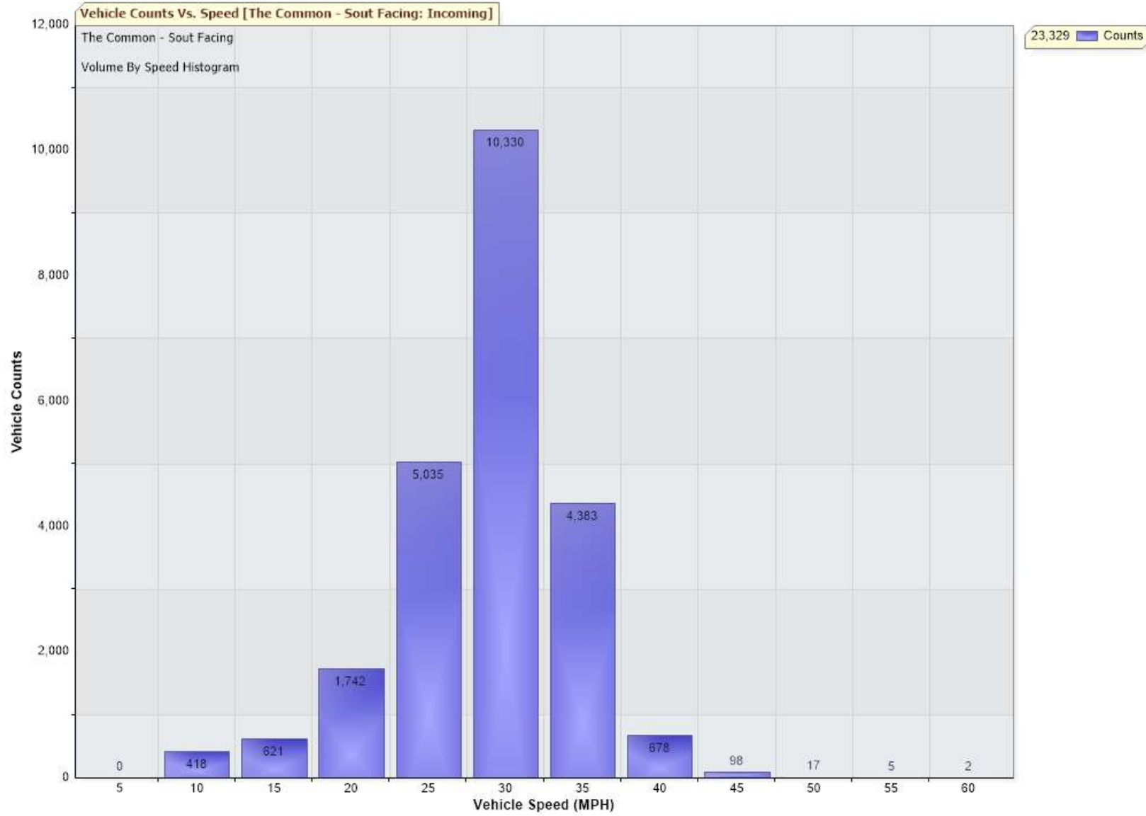
Chart to show vehicle count v speed at The Common between 4 January & 2 February 2024
