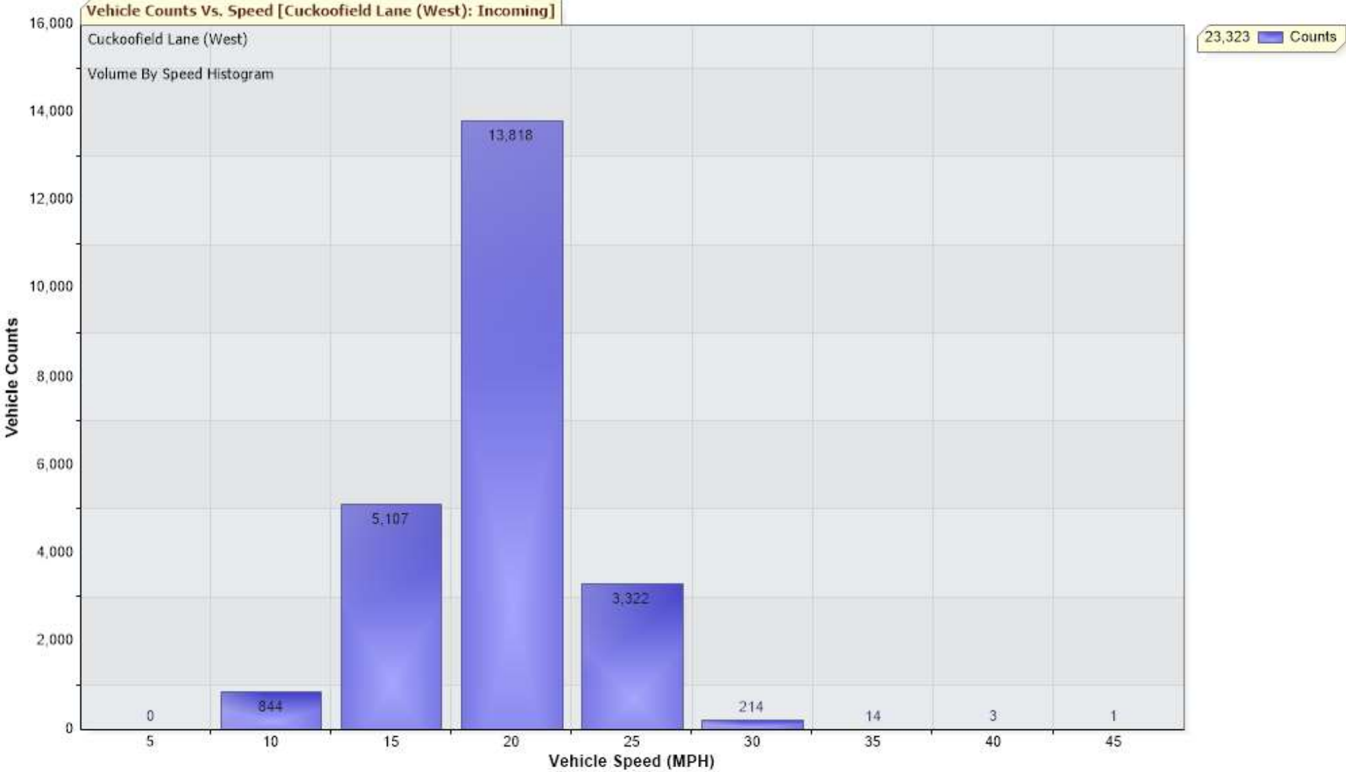
Chart to show vehicle count v speed at Cuckoofield Lane (West) between 22 July & 11 August 2024
