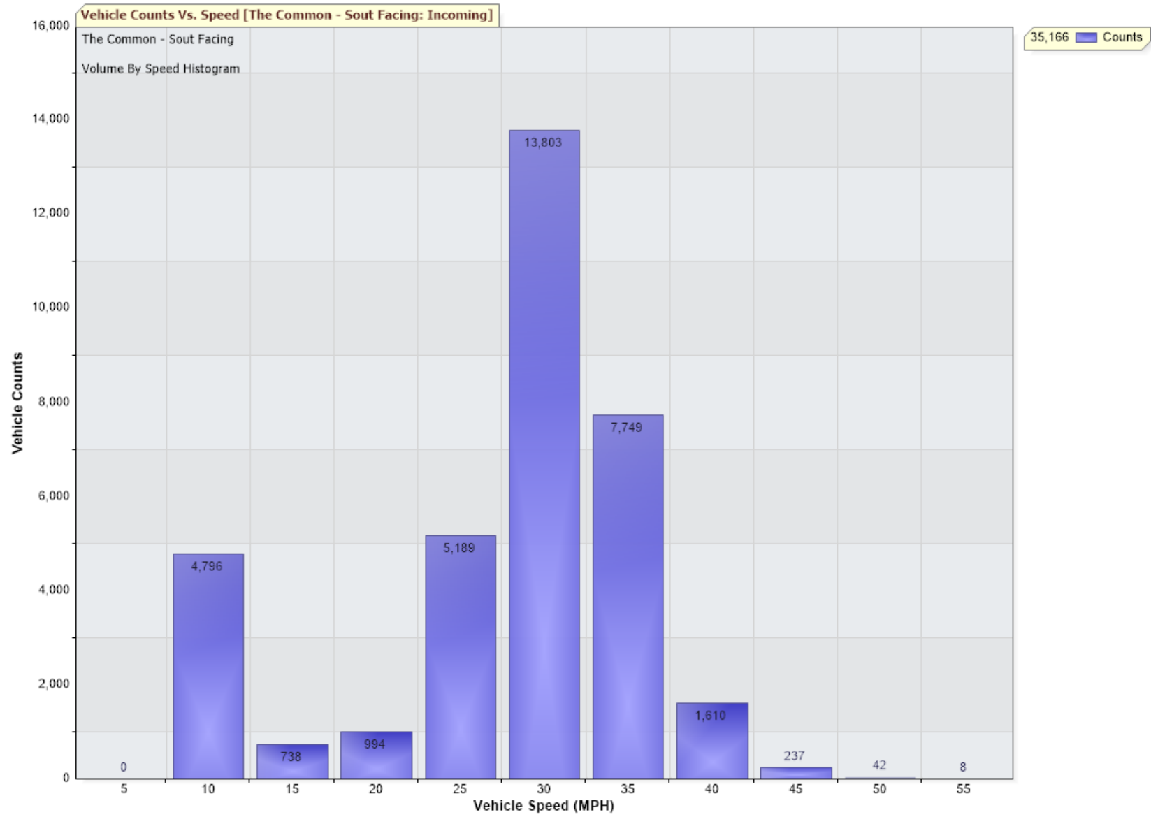
Chart to show vehicle count v speed at The Common between 11 October and 3 November 2023
