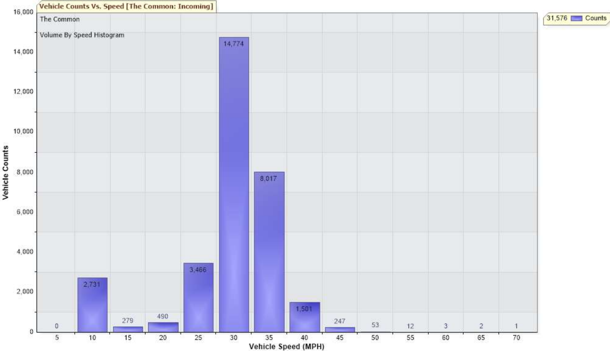
Chart to show vehicle count v speed at The Common (North) between 30 June and 22 July 2024
