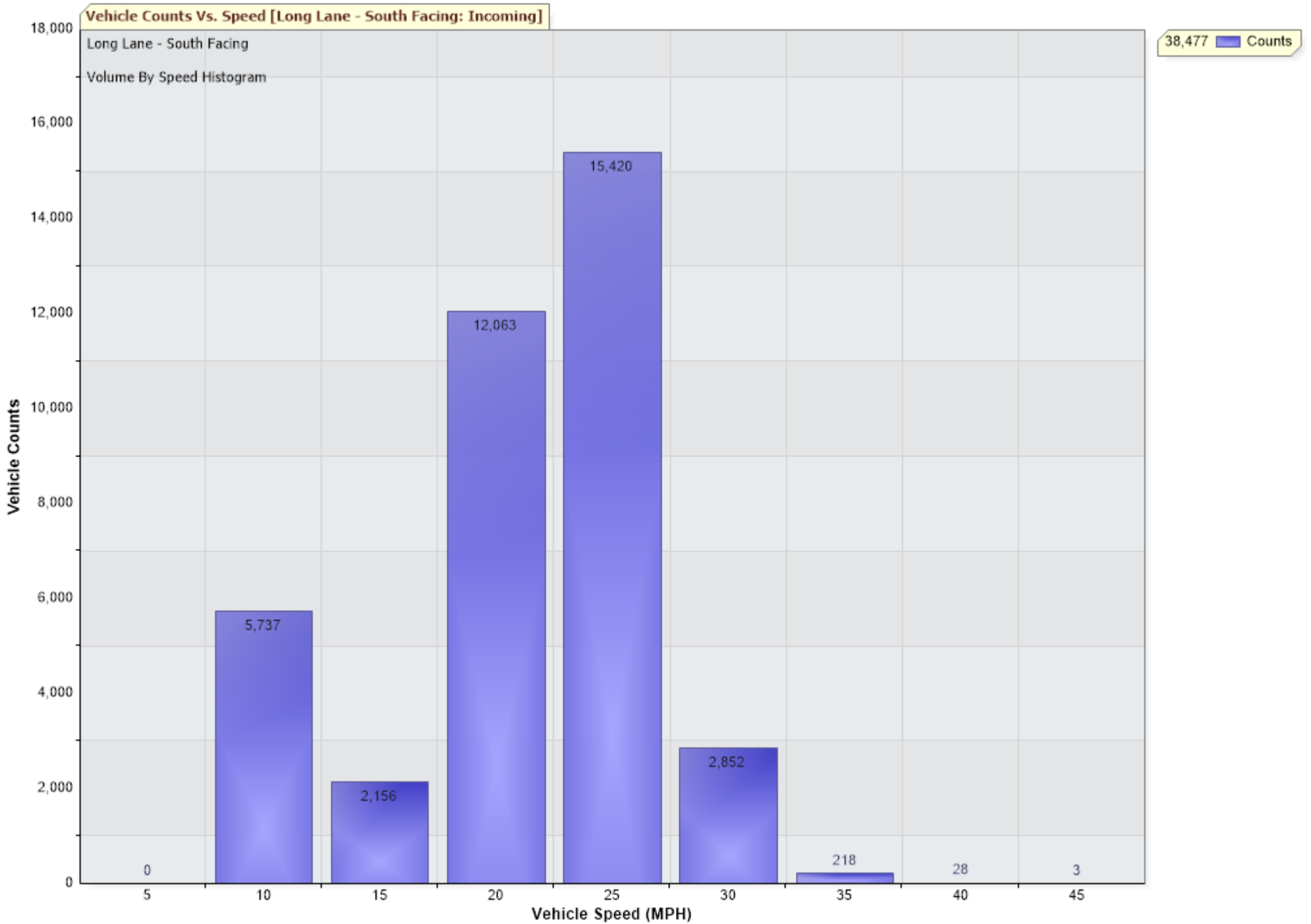
Chart to show vehicle count v speed at Long Lane (South) between 13 July and 10 August 2023
