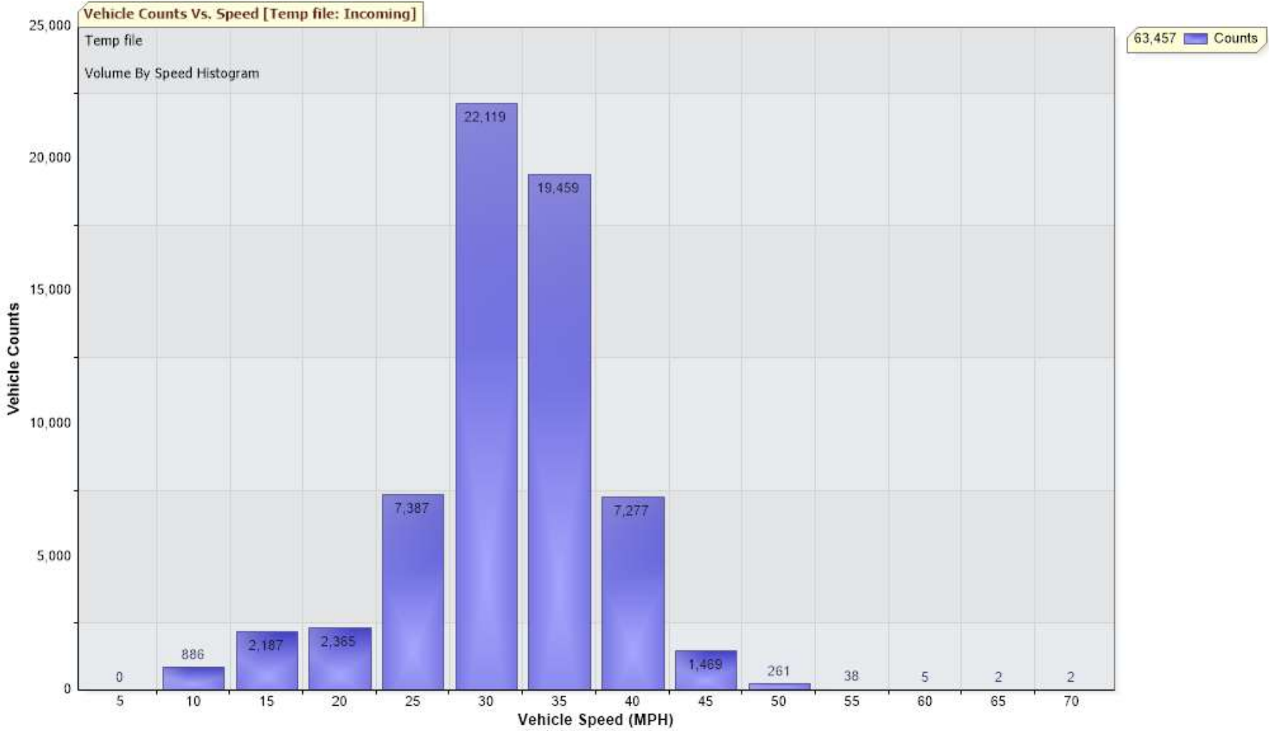
Chart to show vehicle count v speed at Norwich Road between 9 and 30 June 2024
