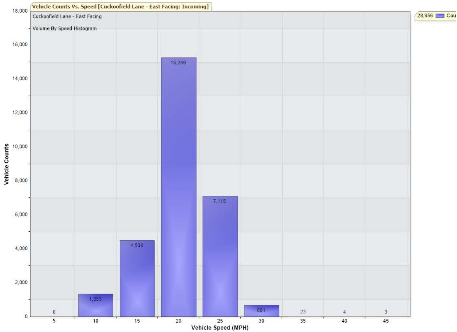
Chart to show vehicle count v speed at Cuckoofield Lane (East) between 11 & 28 August 2023
