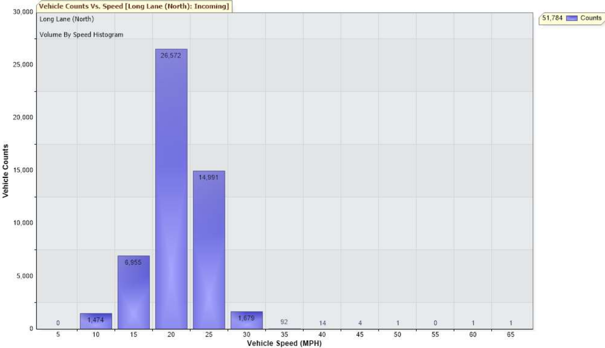
Chart to show vehicle count v speed at Long Lane (North facing) between 11 August and 2 September 2024
