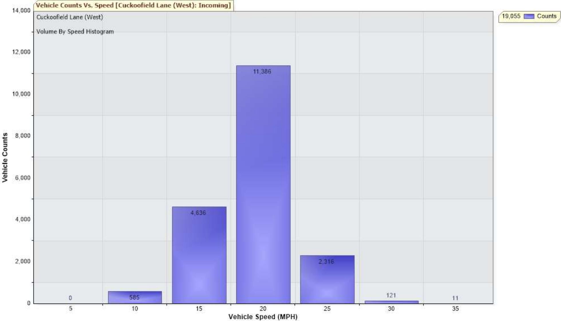
Chart to show vehicle count v speed at Cuckoofield Lane (West) between 27 October & 16 November 2024
